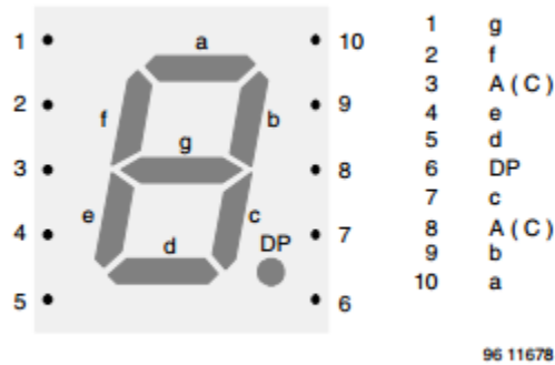
Figure 3 Seven segment display data for TDSG3150.
