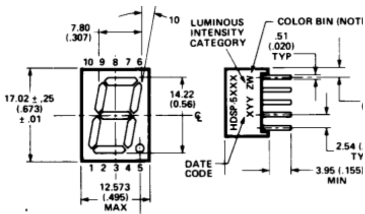
Figure 4 Seven segment display data for HDSP-5601 (along with table) from datasheet.
