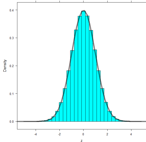
Figure 3 A Gaussian distribution is superimposed on a 1e6 sample distribution histogram.
