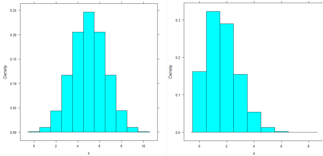
Figure 7: Binomial Distributions for ten coins with 1:1 and 1:5 odds.
